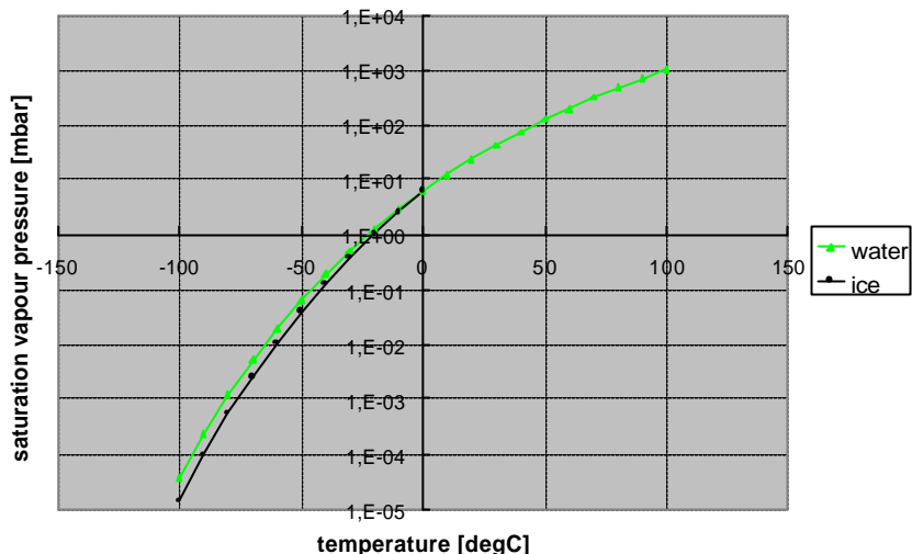
Fig.3 : Vapour saturation curves above ice and water. Below the triple point (0.01 degC) the curve splits into two graphs.
