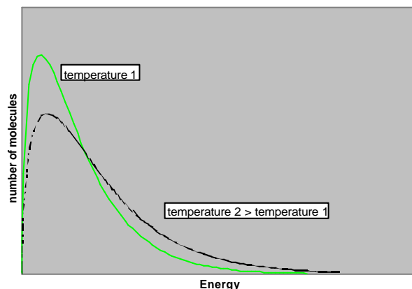
Fig.1: Statistical energy distribution of molecules in a liquid.
